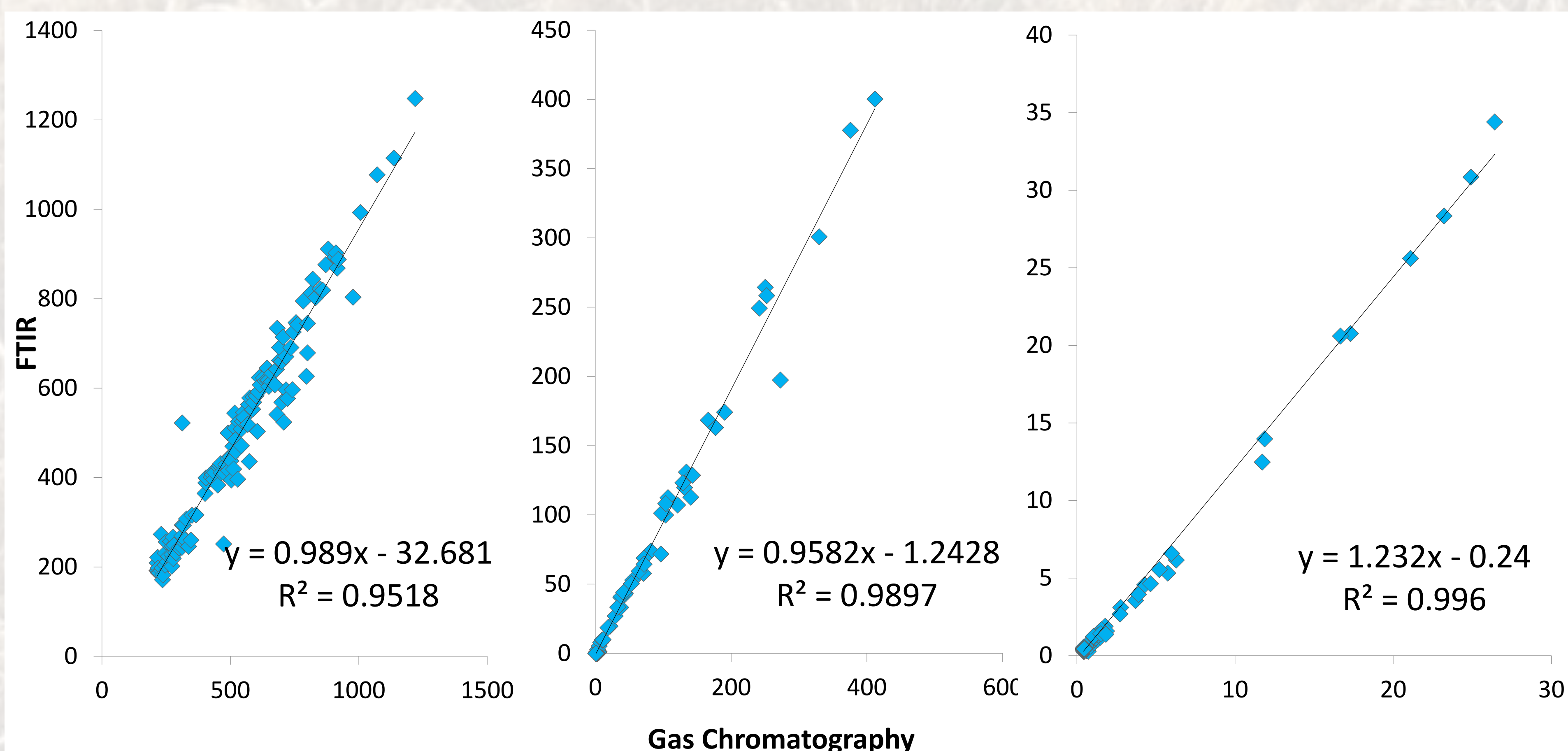
Figure 2. CO 2 , CH 4 , and N 2 O concentration comparisons from 133 paired GHG measurements from FTIR (y-axis) and GC (x-axis).
